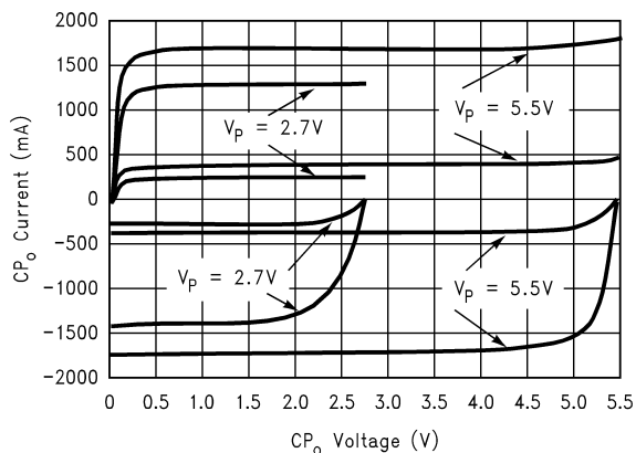
Charge Pump Current vs CP_O Voltage CP_WORD = 0011 and 1111
