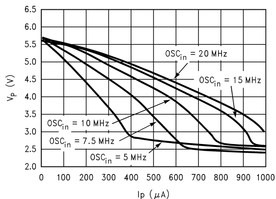
LMX2353 V_P Voltage vs V_P Load Current in V Doubler Mode, T = 25^{\circ}\text{C}
